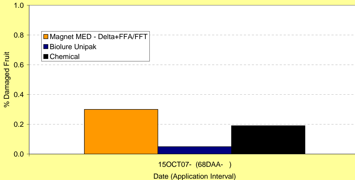
Fruit Damage due to Medfly Attack in Plots with Different Control Tactics - Spain 2007 - Trial 2 (Fortuna, Murcia)
